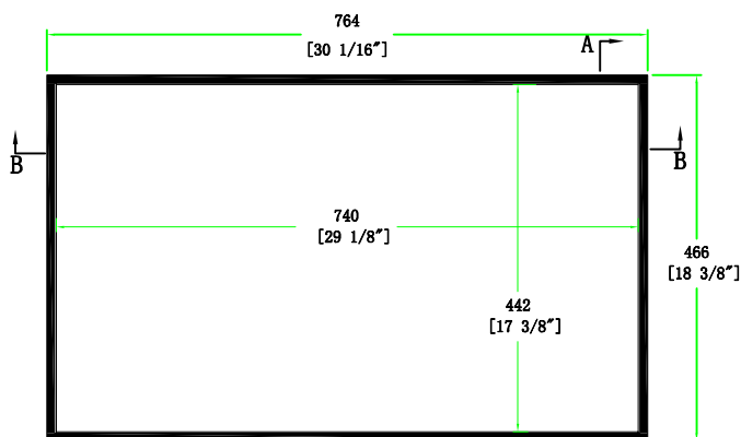
TOP VIEW OF COVER
