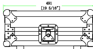
LEFT VIEW
