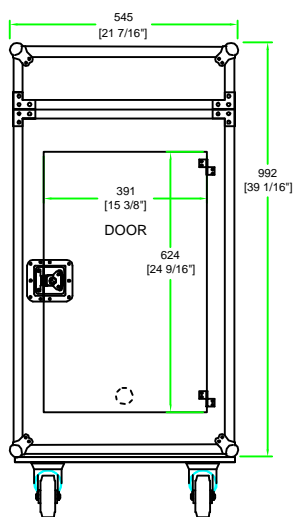
BACK VIEW
