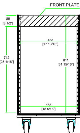
INSIDE VIEW
