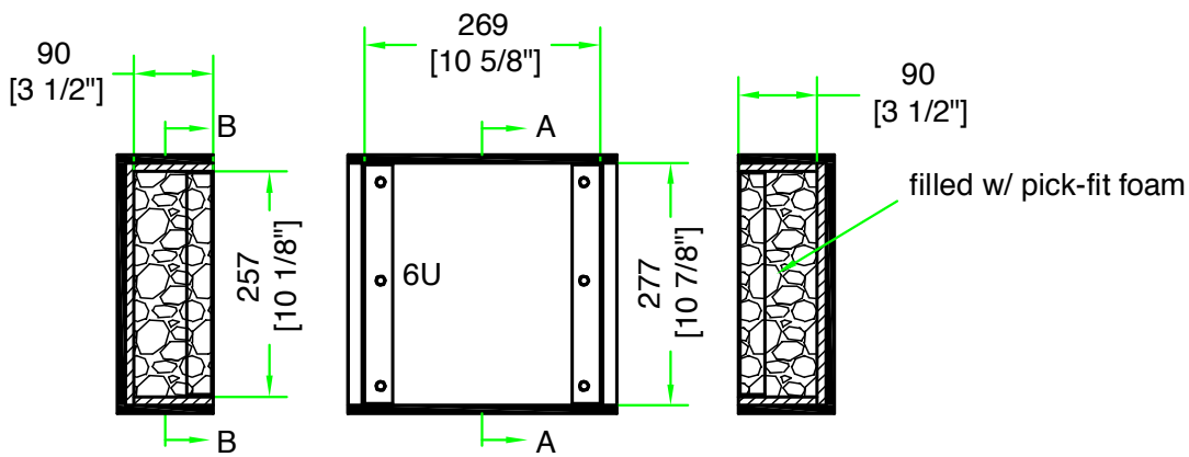
CUTAWAY VIEW
