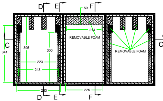
TOP VIEW OF BASE
