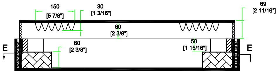
D-D VIEW
