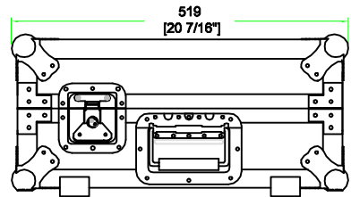
LEFT VIEW
