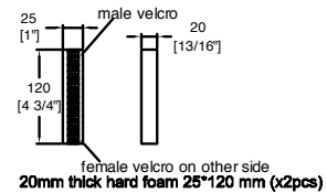
20mm thick hard foam 25*120 mm (x2pcs)
