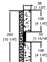
F-F VIEW
