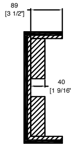
D-D VIEW
