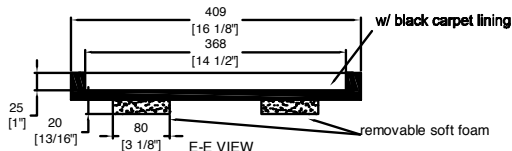
E-E VIEW
