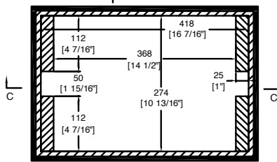
TOP VIEW OF BASE
