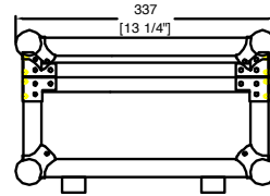
LEFT VIEW
