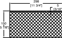
RIGHT VIEW
