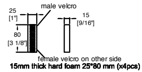
15mm thick hard foam 25*80 mm (x4pcs)
