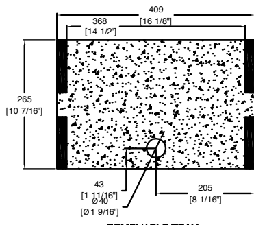
REMOVABLE TRAY
