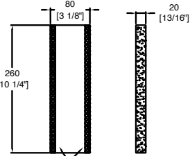
20mm thick soft foam 80*260 mm (x2pcs)
