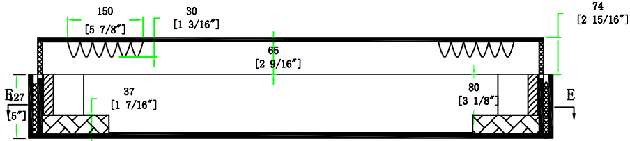
D-D VIEW
