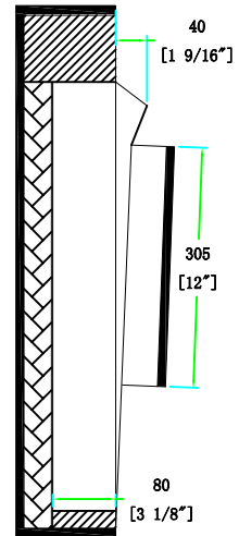
C-C VIEW
