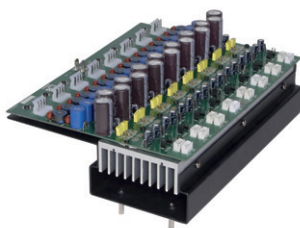
POW2 Power amplifier kit
