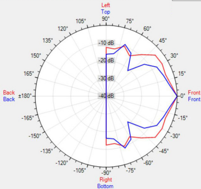
Data Shown: EN-SMS6MT6-W (APart Audio) Display Parameters: Frequency: 4000Hz (1/24th Octave)
