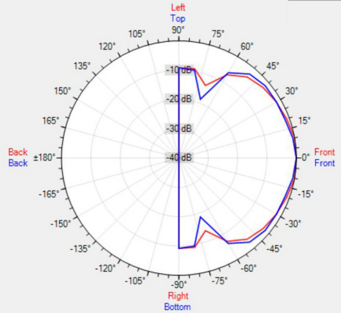
Data Shown: EN-SMS6MT6-W (APart Audio) Display Parameters: Frequency: 2000Hz (1/24th Octave)
