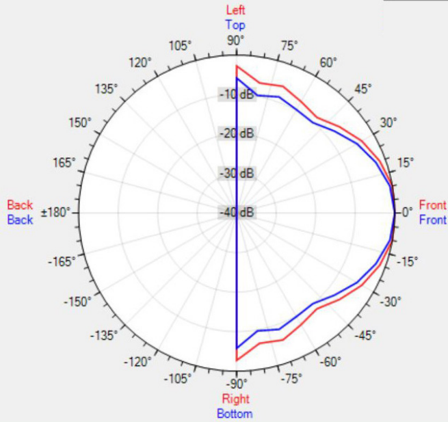
Data Shown: EN-SMS6MT6-W (APart Audio) Display Parameters: Frequency: 1000Hz (1/24th Octave)
