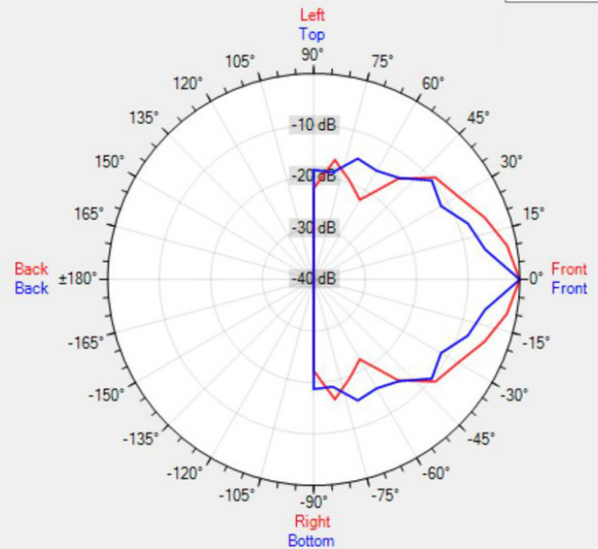
Data Shown: EN-SMS6MT6-W (APart Audio) Display Parameters: Frequency: 8000Hz (1/24th Octave)
