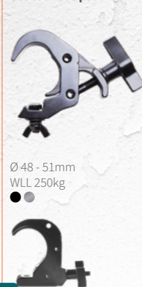
Selflock coupler
