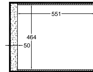
D-D VIEW
