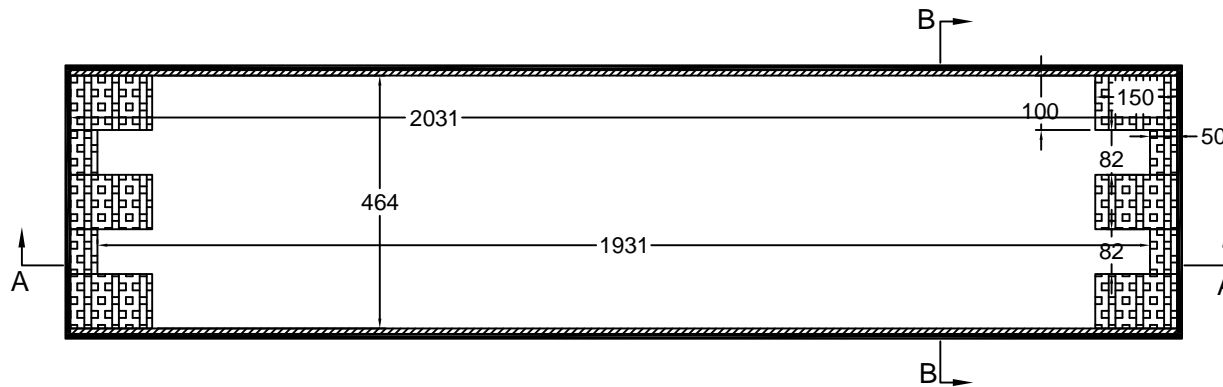
TOP VIEW OF BASE
